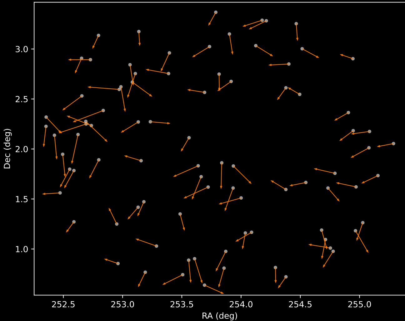
APOGEE DR17 Cluster 2 Proper Motion Vectors (n=86)
