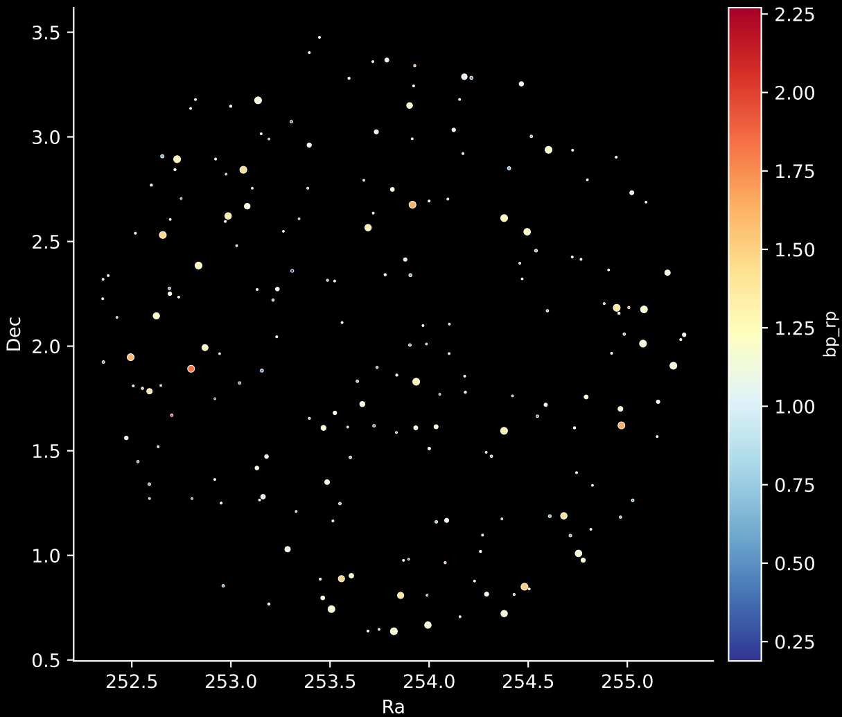
APOGEE DR17 Field: [240+45] Stars: 202
