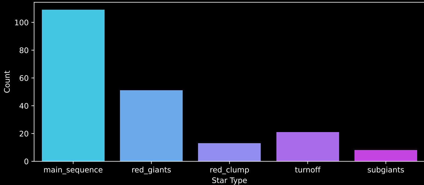
APOGEE DR17 Field: [240+45] Count plot of Star Type
