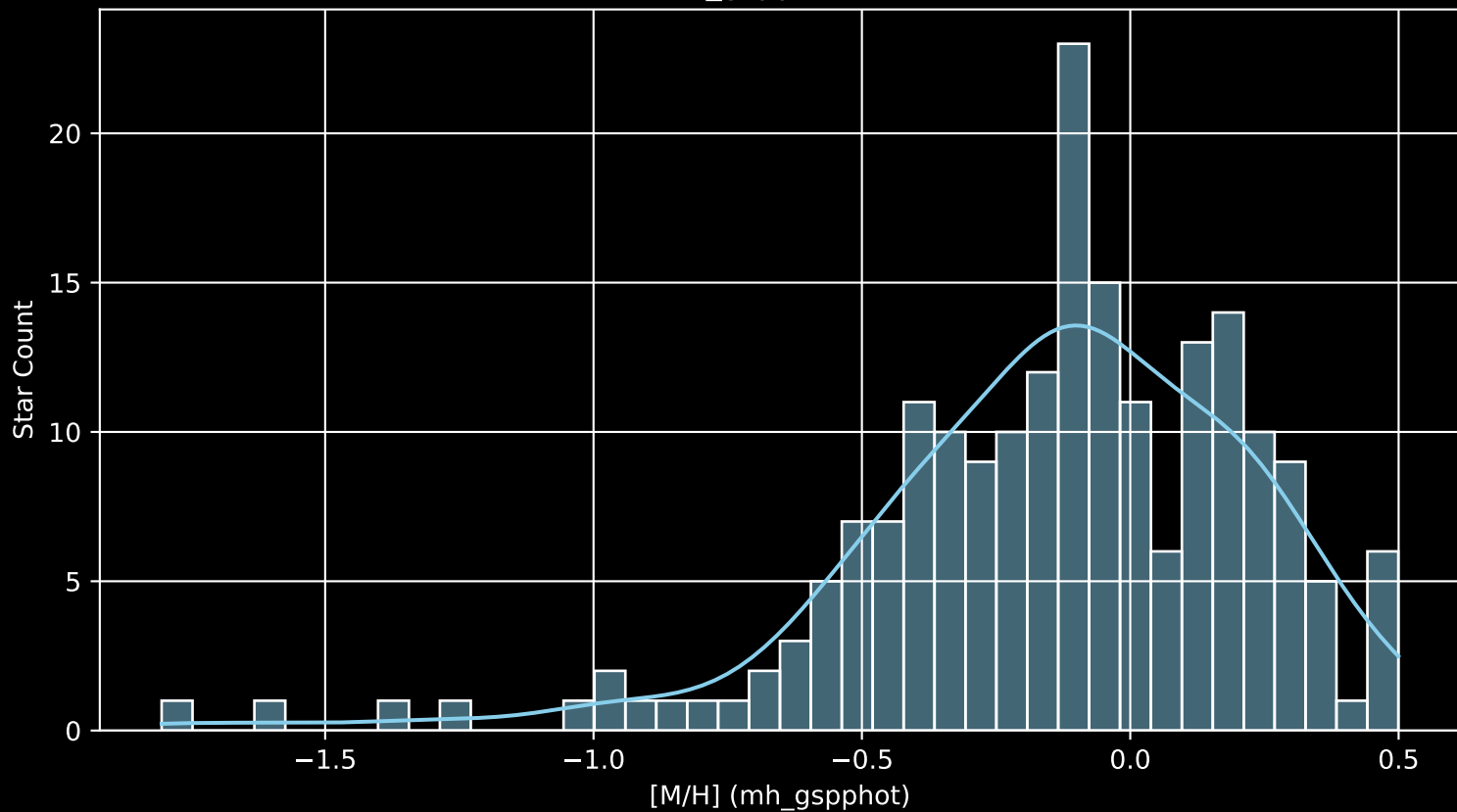
APOGEE DR17 Field: [240+45 [M/H] (mh_gspphot) (n= 200)
