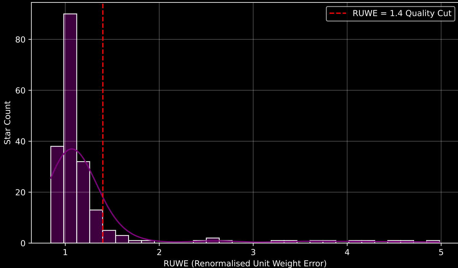
GAPOGEE DR17 Field [240+45] RUWE Distribution (n= 196)
