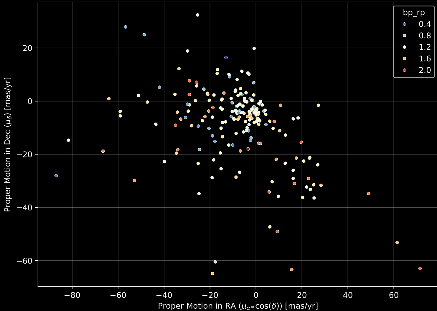
APOGEE DR17 Field: [240+45] Proper Motion Diagram (n= 202)
