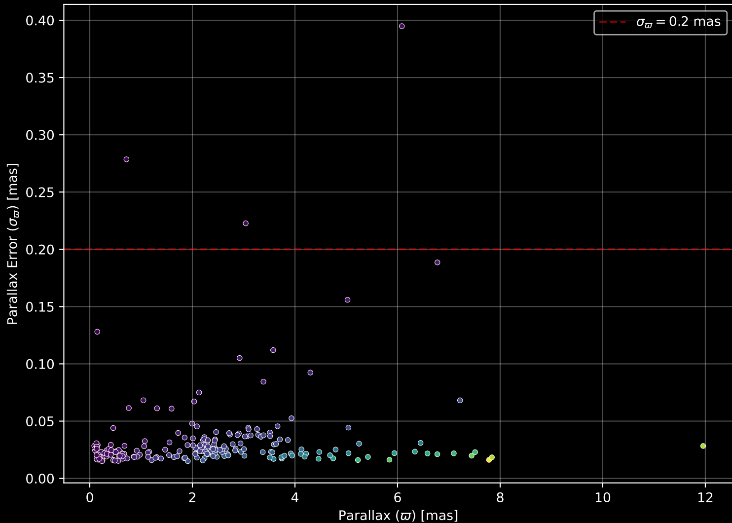
APOGEE DR17 Field: [240+45] Parallax Quality (n= 202)
